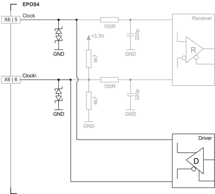
Figure 3-22 SSI absolute encoder clock output
