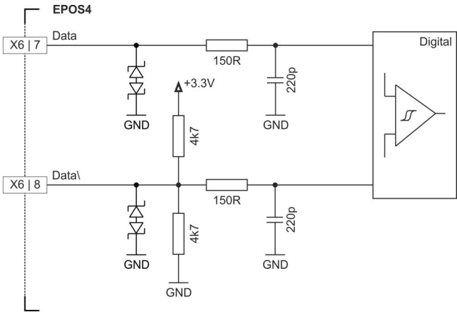
Figure 3-21 SSI absolute encoder data input
