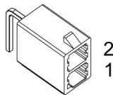
Figure 3-6 Power supply connector X1
