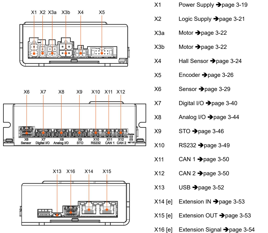
Figure 3-5 Connectors
