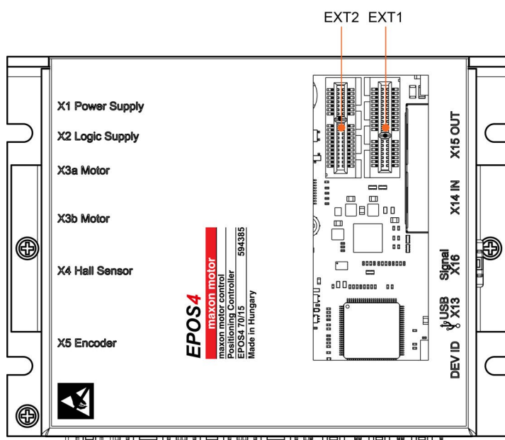
Figure 3-43 Extension slots
