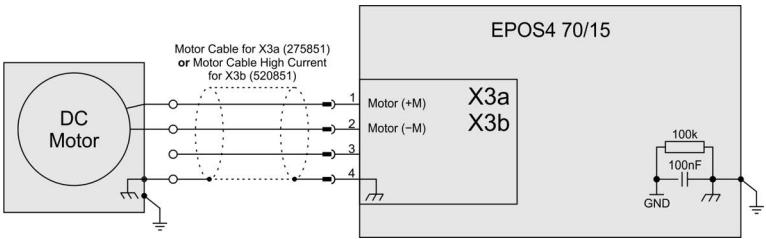
Figure 4-50 DC motor
