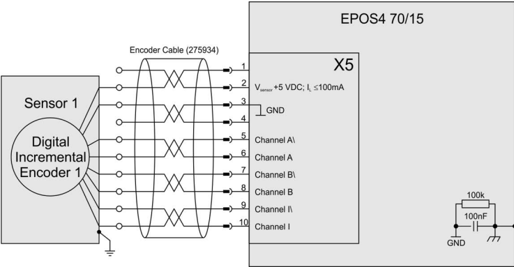
Figure 4-53 Digital incremental encoder 1 (Sensor 1)
