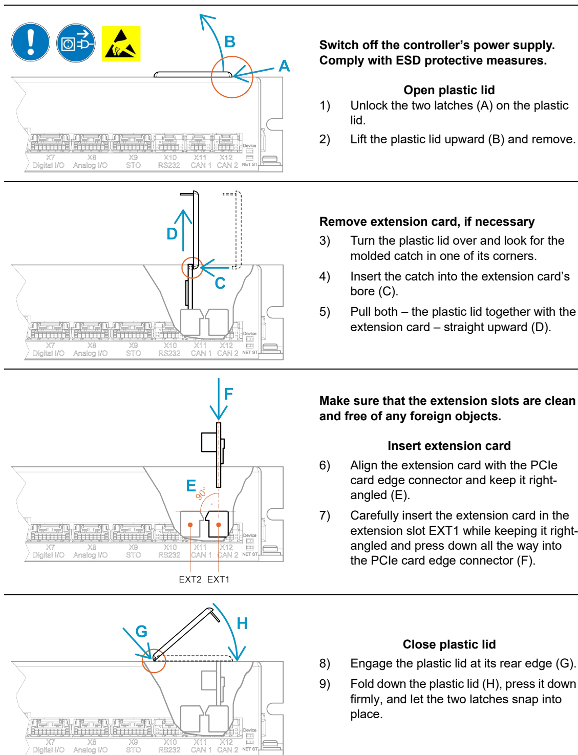
Figure 3-44 Installation & removal of an extension card
