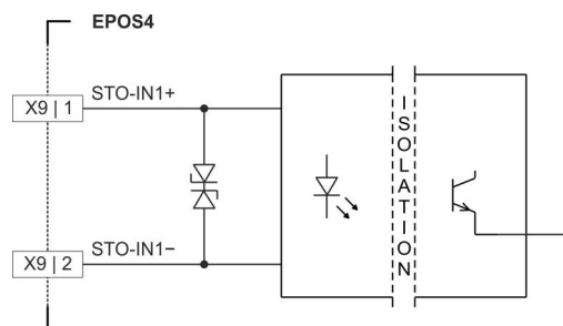
Figure 3-36 STO-IN1 circuit (analogously valid for STO-IN2)
