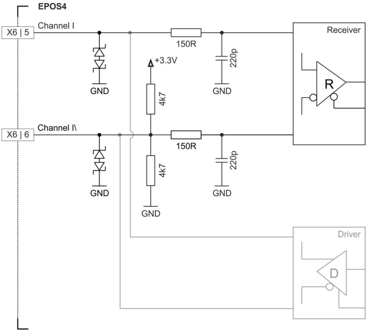
Figure 3-16 Digital incremental encoder input circuit Ch I
